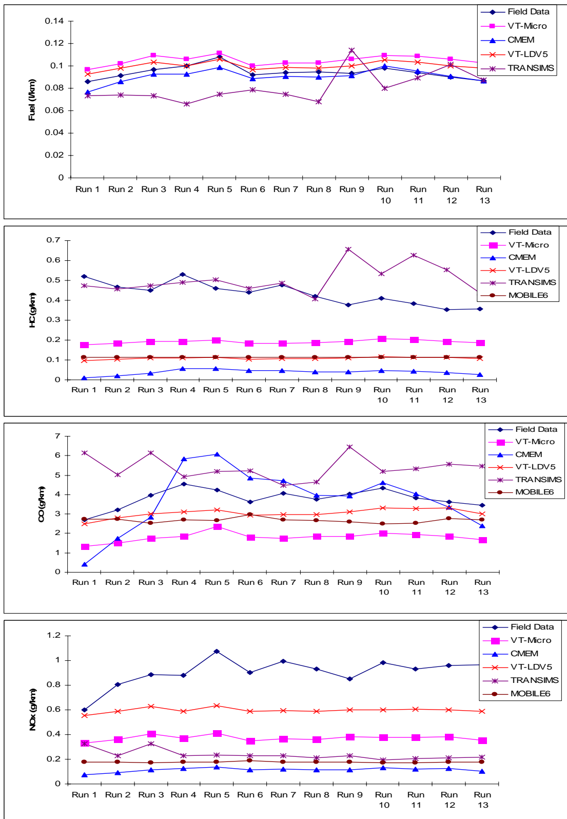
Figure 4. The Emission Estimate in TRANSIMS, MOBILE6, CMEM, VT-Composite versus the OEM data
